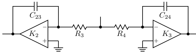
Figure 44: Showing the result of two invocations of the fbfilter macro, with labels.
