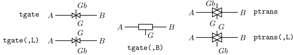
Figure 30: The tgate ( linespec , [B] [R|L]) element, derived from a customized diode and ebox , and the ptrans ( linespec , [R|L]) macro. These are not two-terminal elements, so the linespec argument defines the direction and length of the line from A to B but not the element position.
