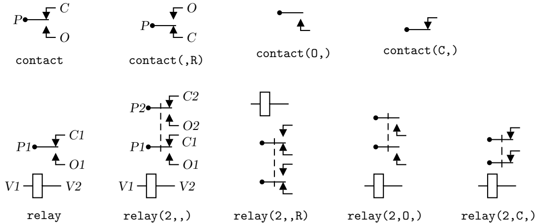
Figure 24: The contact(0|C,R) and relay(poles,0|C,R) macros (default direction right).
