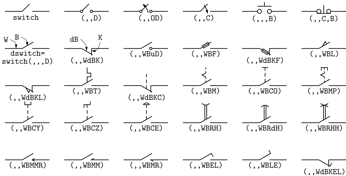
Figure 9: The basic switch( linespec ,L|R,[O|C][D],B) macro and more elaborate dswitch( linespec ,R,W[ud]B[K]chars) macro, with drawing direction right . Setting the second argument to R produces a mirror image with respect to the drawing direction. The macro switch(,,D) is a wrapper for the comprehensive dswitch macro.
