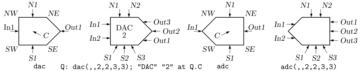
Figure 40: The dac(width,height,nIn,nN,nOut,nS) and adc(width,height,nIn,nN,nOut,nS) macros.
