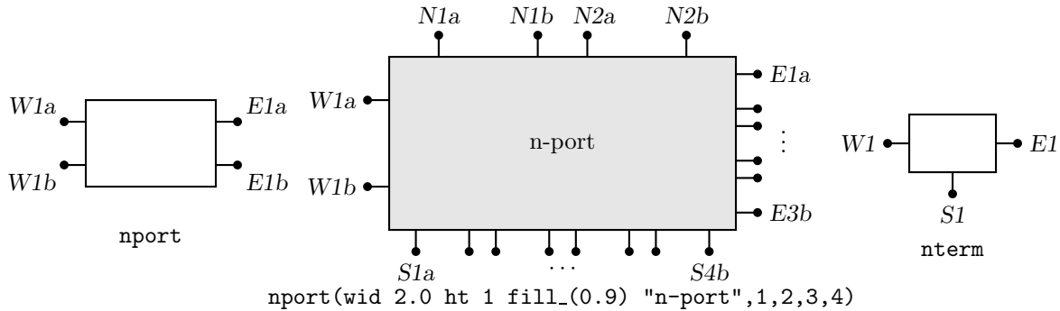
Figure 21: The nport macro draws a sequence of pairs of named pins on each side of a box. The pin names are shown. The default is a twoport. The nterm macro draws single pins instead of pin pairs.
